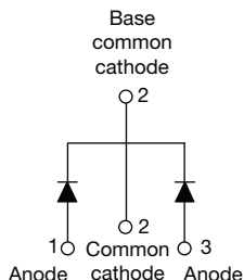
VS-MBRB30..CT-M3
