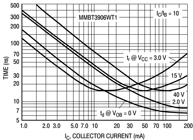
Figure 24. Turn-On Time
