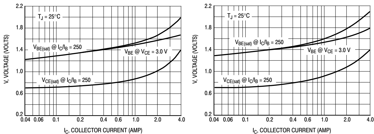
Figure 11. "On" Voltages
