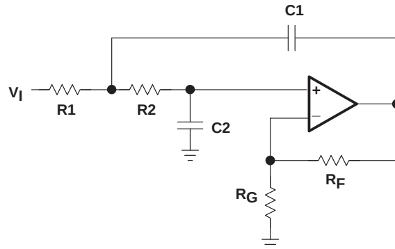
Figure 38. 2-Pole Low-Pass Sallen-Key Filter
