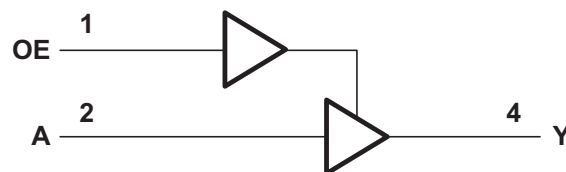
Simplified Schematic
