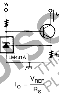
Figure 16. Constant-Current Sink
