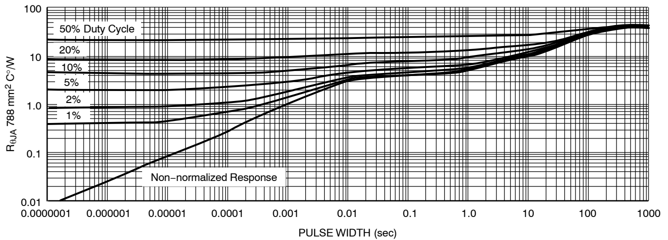
Figure 58. Duty Cycle for 1" Spreader Boards, D²PAK 5-Lead
