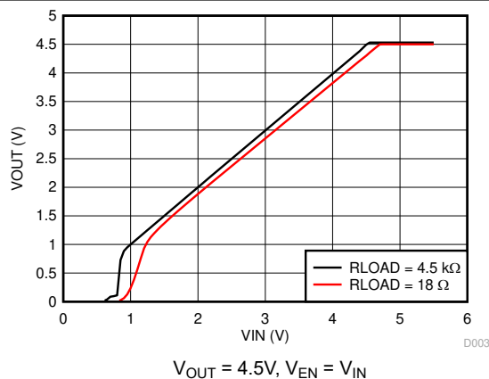
Figure 5-4. V_{OUT} vs V_{IN}
