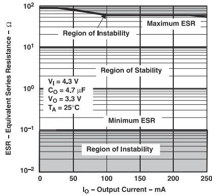
Figure 5-52. Typical Region of Stability ESR vs Output Current (Legacy Chip)
