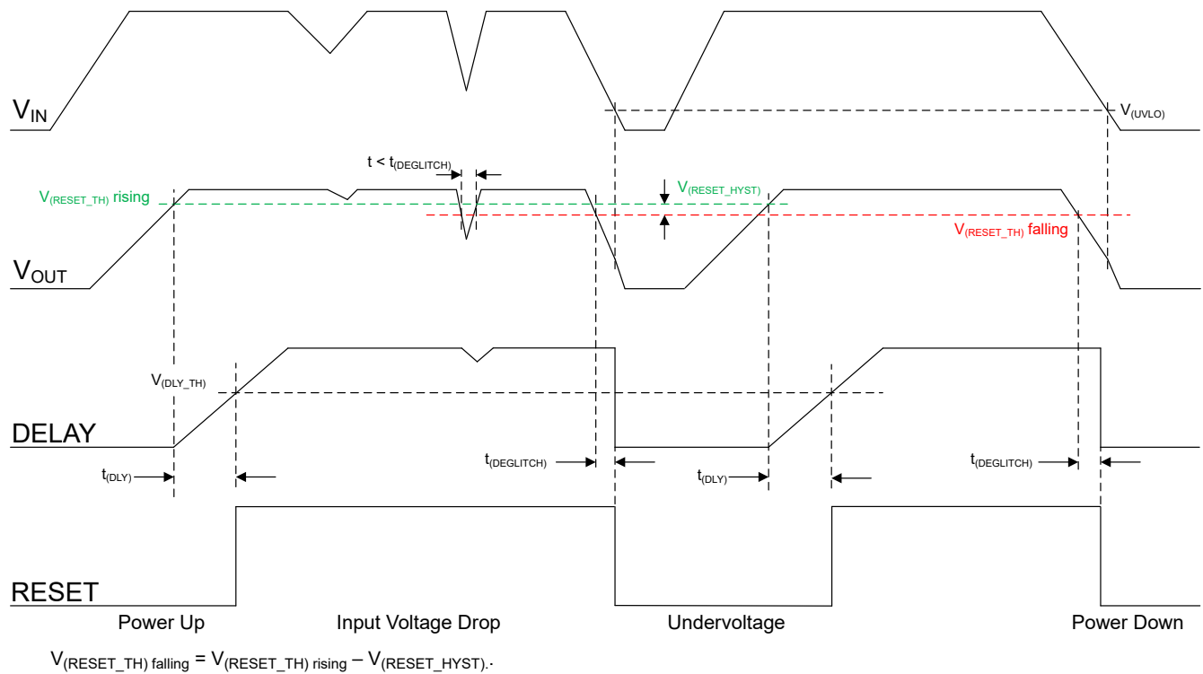
Figure 5-2. Typical Power-Good RESET Timing Diagram (New Chip)
