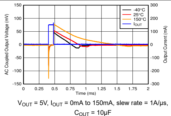
Figure 5-44. Load Transient, No Load to 150mA (New Chip)
