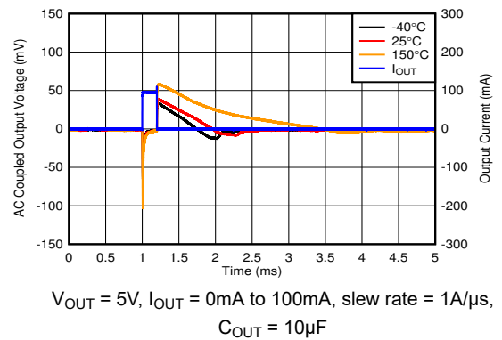
Figure 5-40. Load Transient, No Load to 100mA (New Chip)
