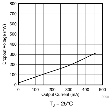
Figure 5-19. Dropout Voltage ( V_{DO} ) vs Output Current (Legacy Chip)
