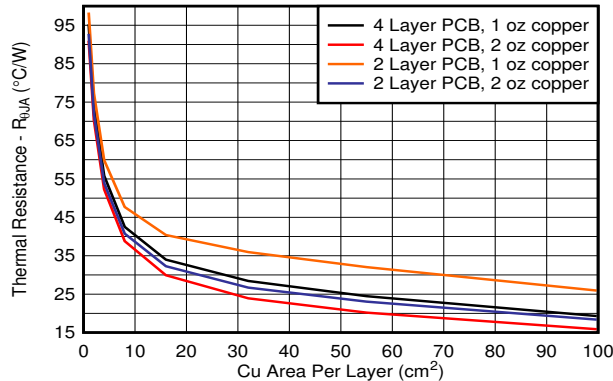
Figure 8-2. R_{\theta JA} vs Copper Area (KVU Package)
