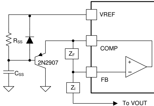
Figure 7-6. Soft-Start Implementation
