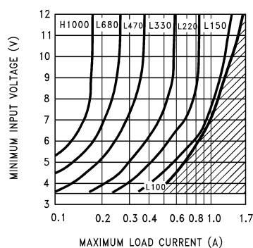
Figure 35. LM2577-15 Inductor Selection Guide
