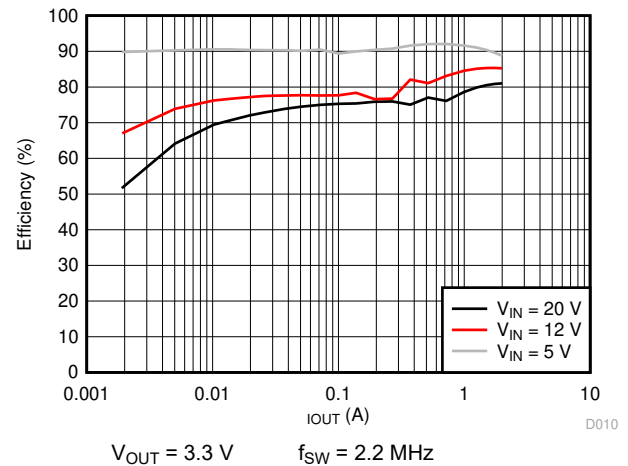
Figure 5-4. Efficiency vs. Load Current
