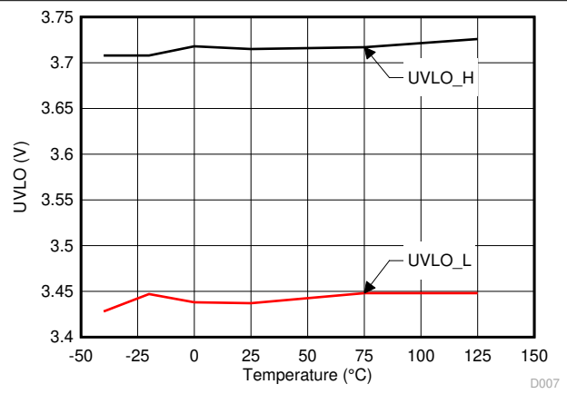
Figure 5-12. UVLO Threshold
