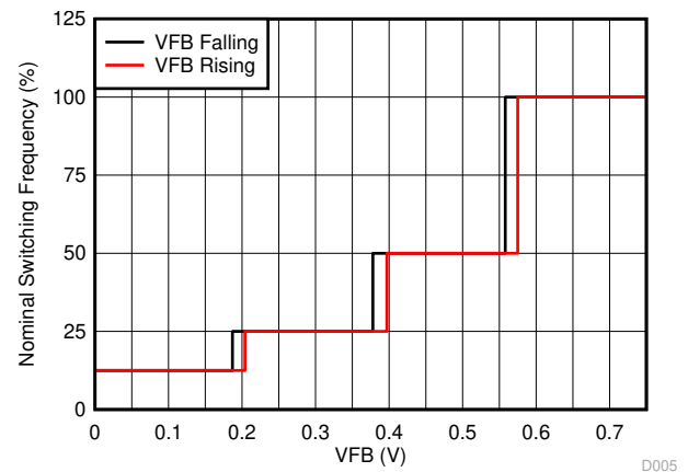
Figure 5-6. Frequency vs V_{FB}
