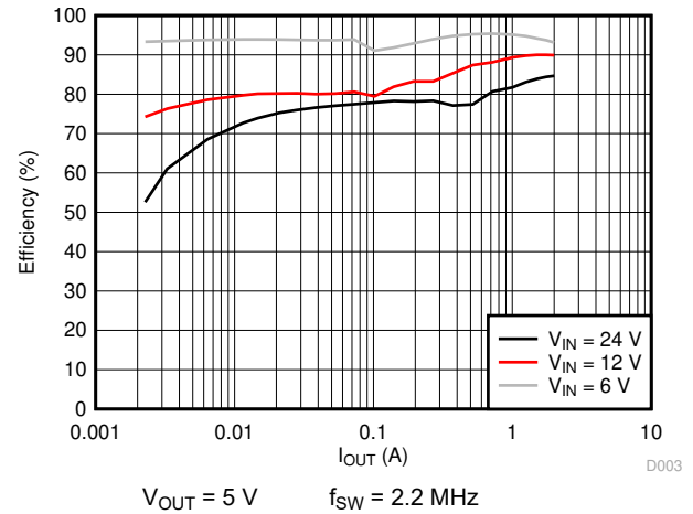
Figure 5-2. Efficiency vs. Load Current
