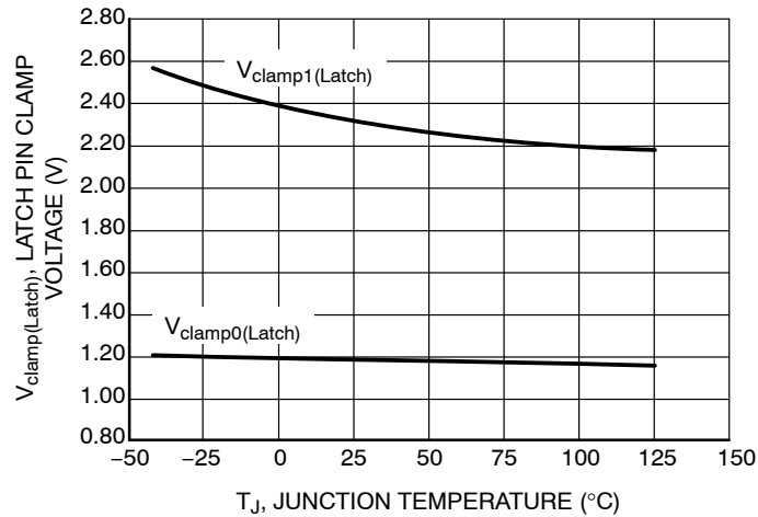
Figure 42. Latch Pin Clamp Voltage vs. Junction Temperature
