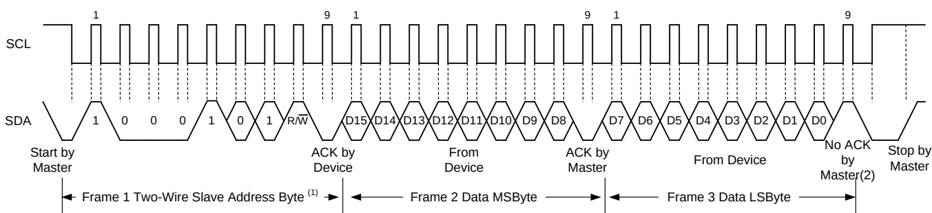
Figure 21. I²C Read Example
