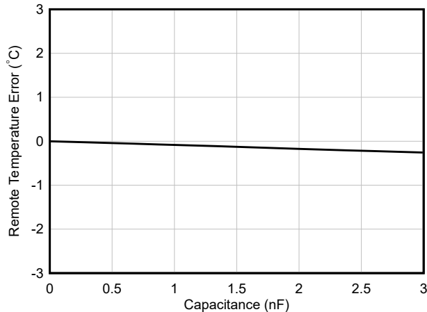
Figure 6-13. Remote Temperature Error vs Differential Capacitance (New Chip)
